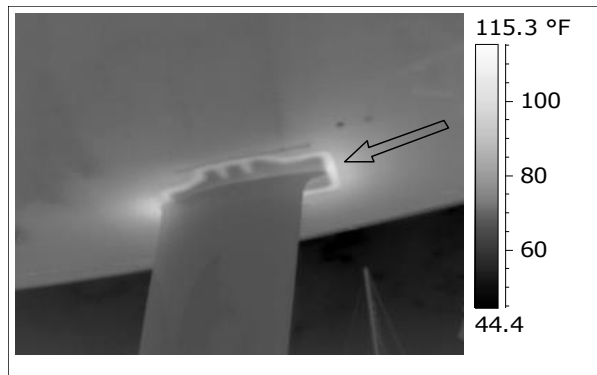
FLIR T440BX
